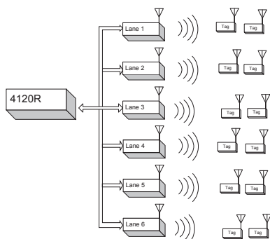
Typical Configuration
