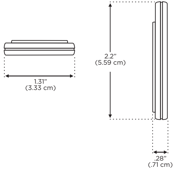
CompacTag™ 2230 Dimensions
