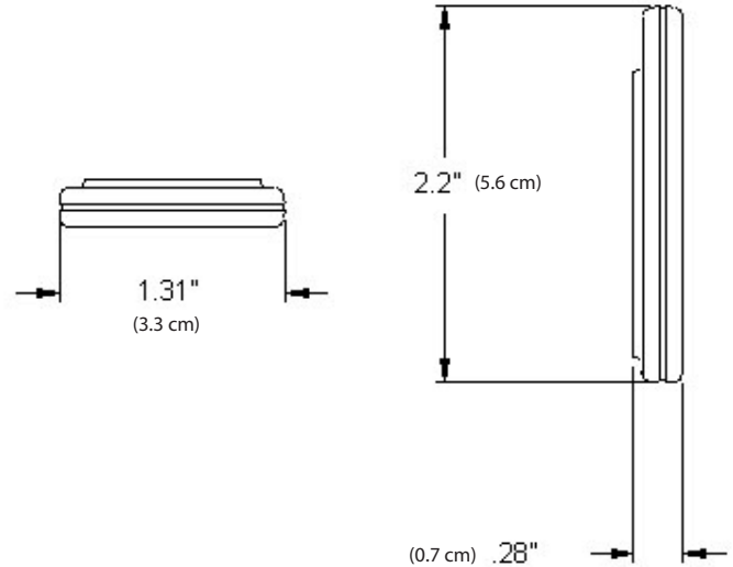
CompacTag™ 2230 Dimensions
